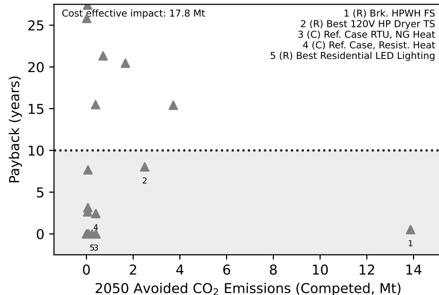
Simple Payback
